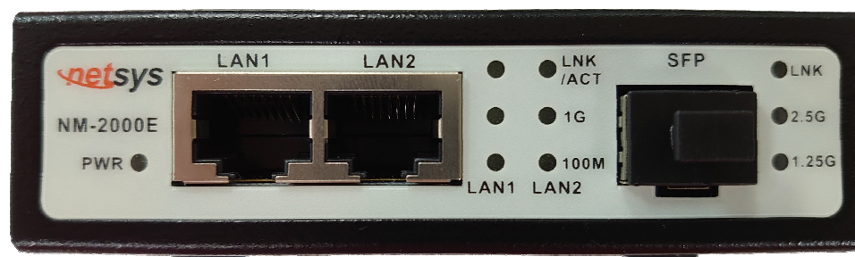
Figure 2.1 Front Panel
