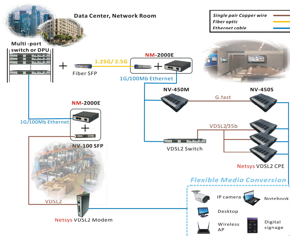
Figure 2.2 Application Diagram
