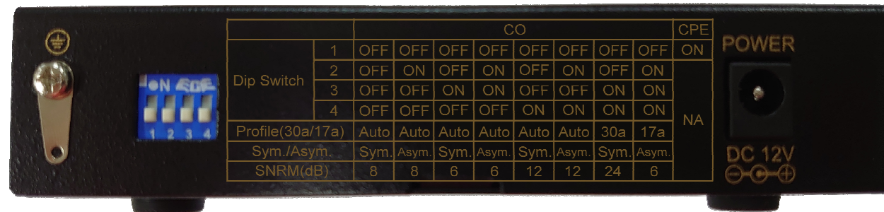
Figure 3.2 Rear Panel
