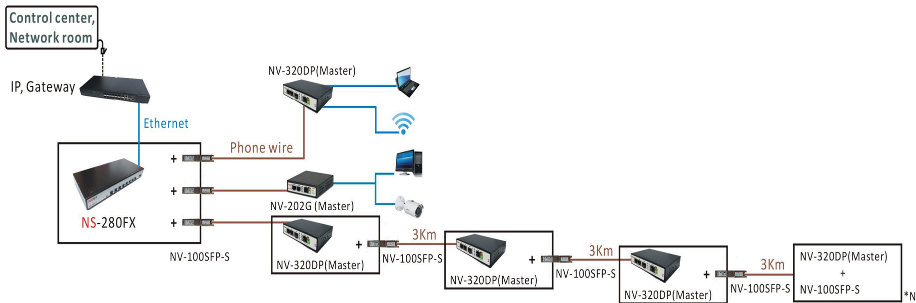
Figure 2.2 Application Diagram
