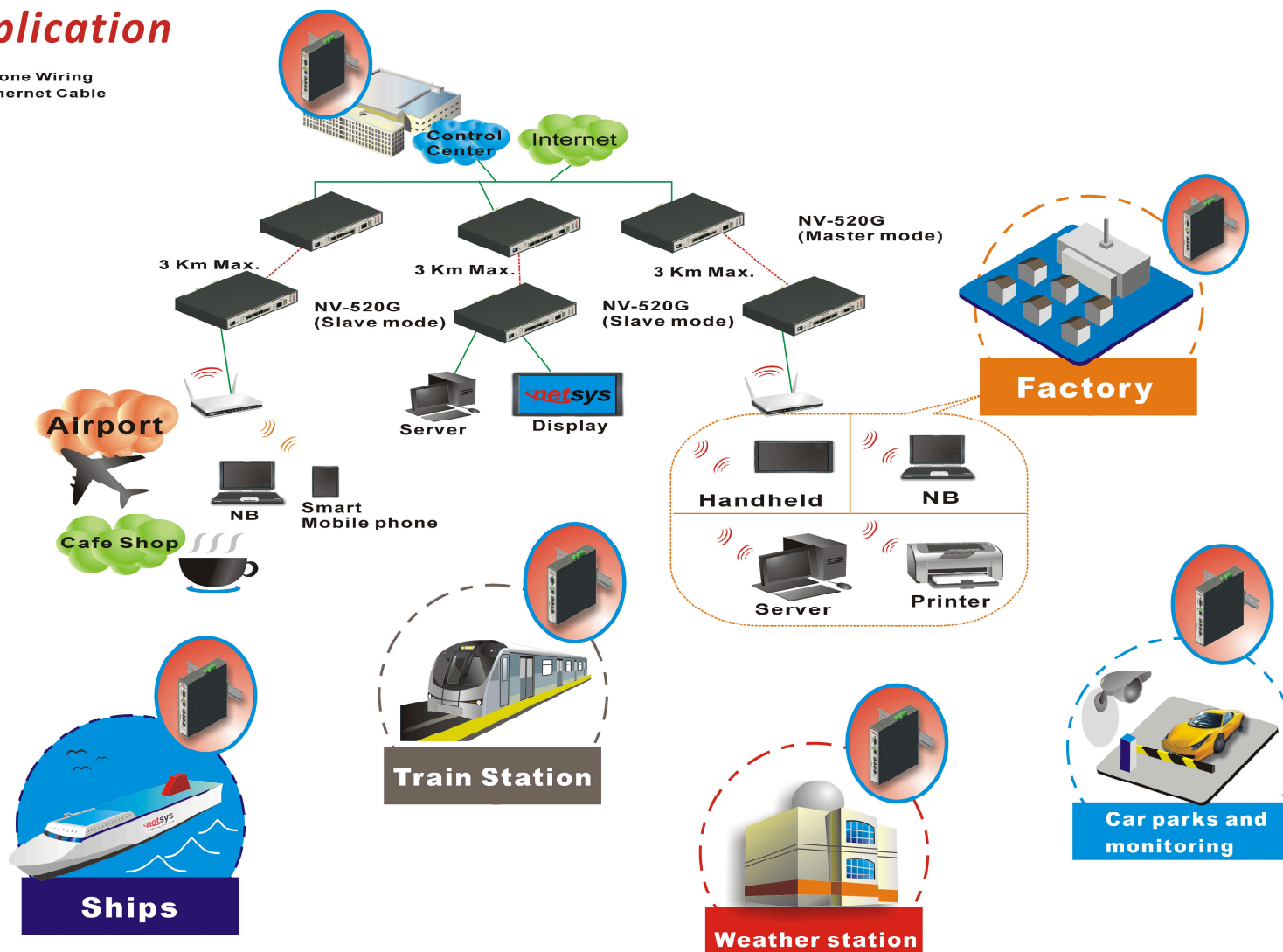
Figure 2.7 NV-520G industrial-grade application
