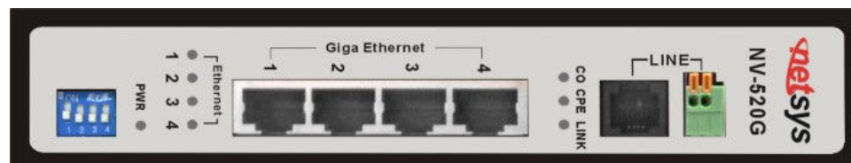
Figure 3.1 Front Panel
